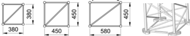
Portalbein
